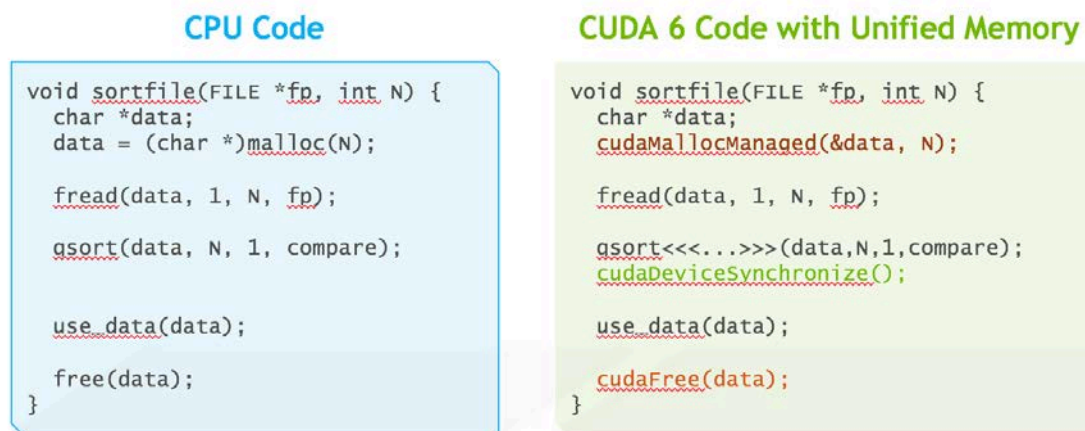
Figure 20. CUDA 6 Unified Memory Simplifies Porting Code to the GPU
