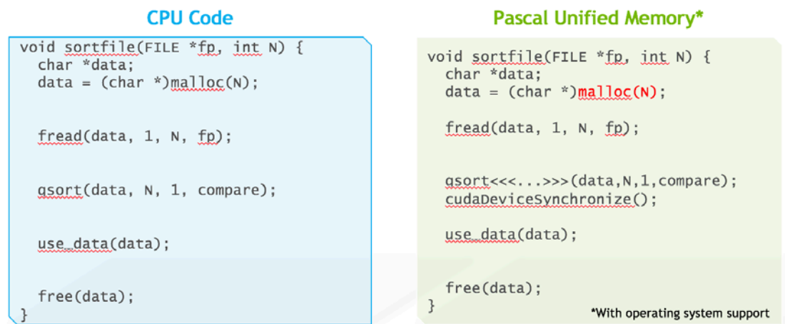
Figure 22. With Operating System Support, Pascal is Capable of Supporting Unified Memory with the Default System Allocator. (Here, malloc is all that is needed to allocate memory accessible from any CPU or GPU in the system.)
