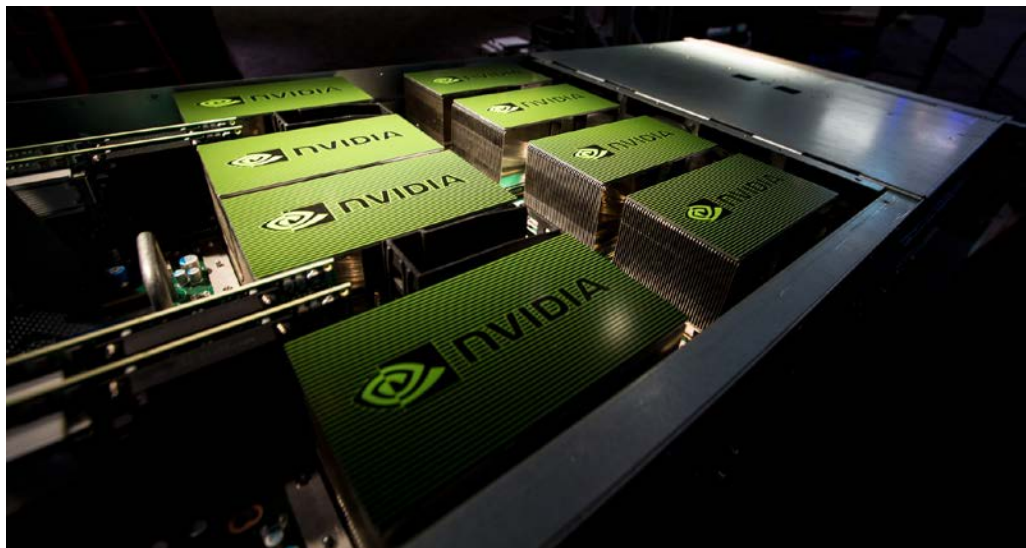
Figure 13. NVIDIA DGX-1 with Eight NVIDIA Tesla P100 GPUs
