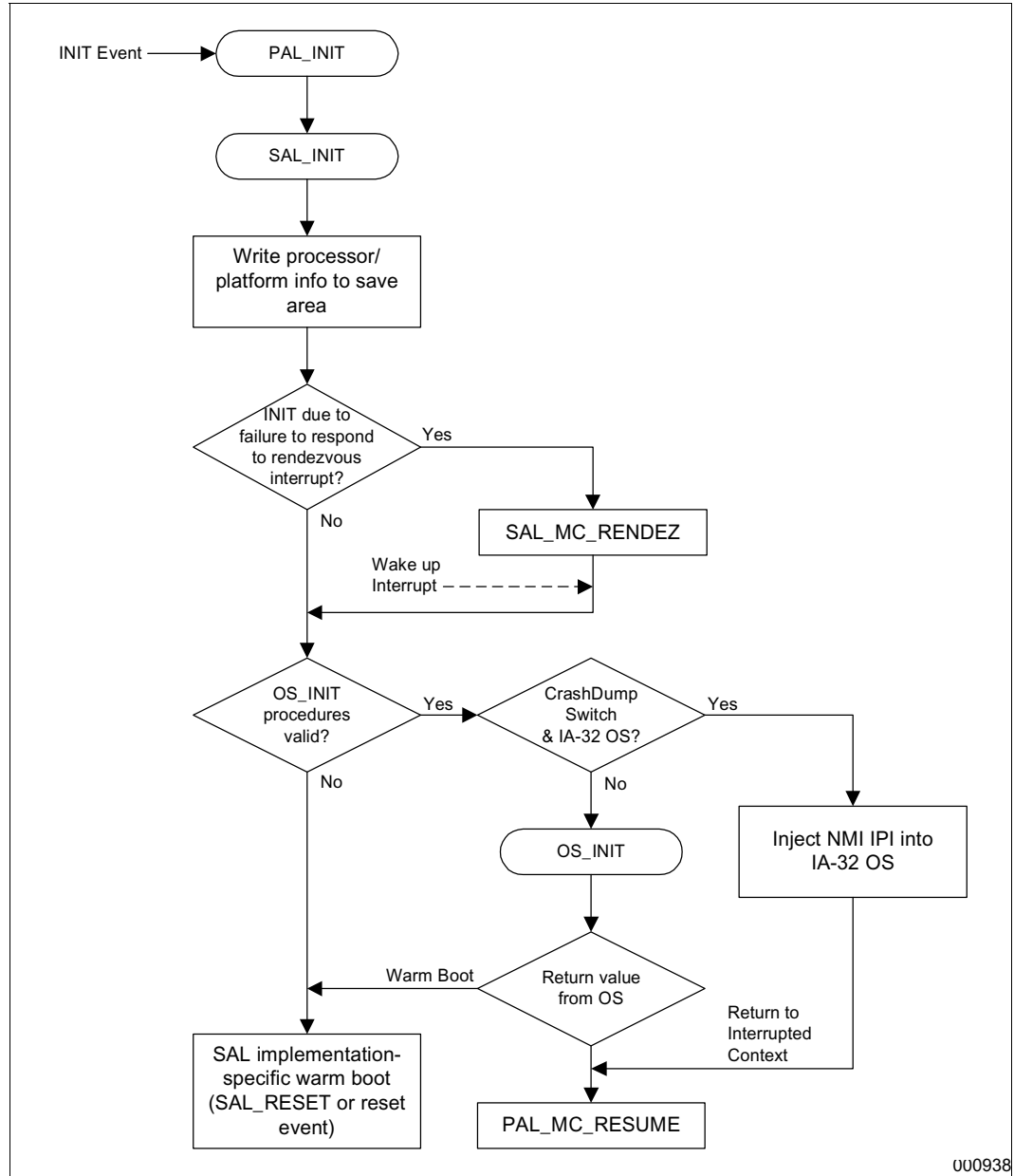
Figure 13-5. INIT Flow
