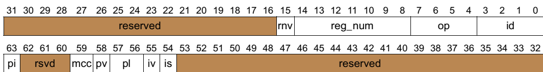
Figure 11-40. Reg_File_Check Layout
