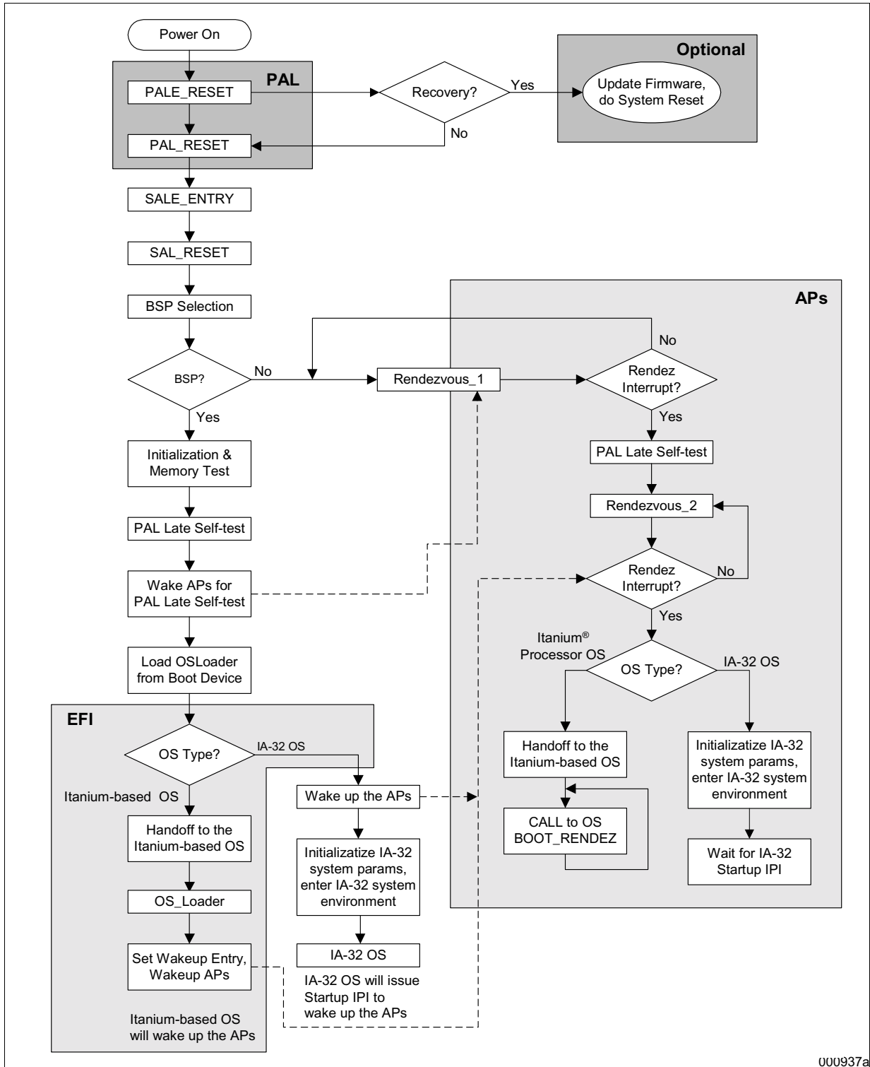
Figure 13-2. Control Flow of Boot Process in a Multi-processor Configuration
