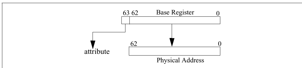
Figure 4-20. Physical Addressing Memory
