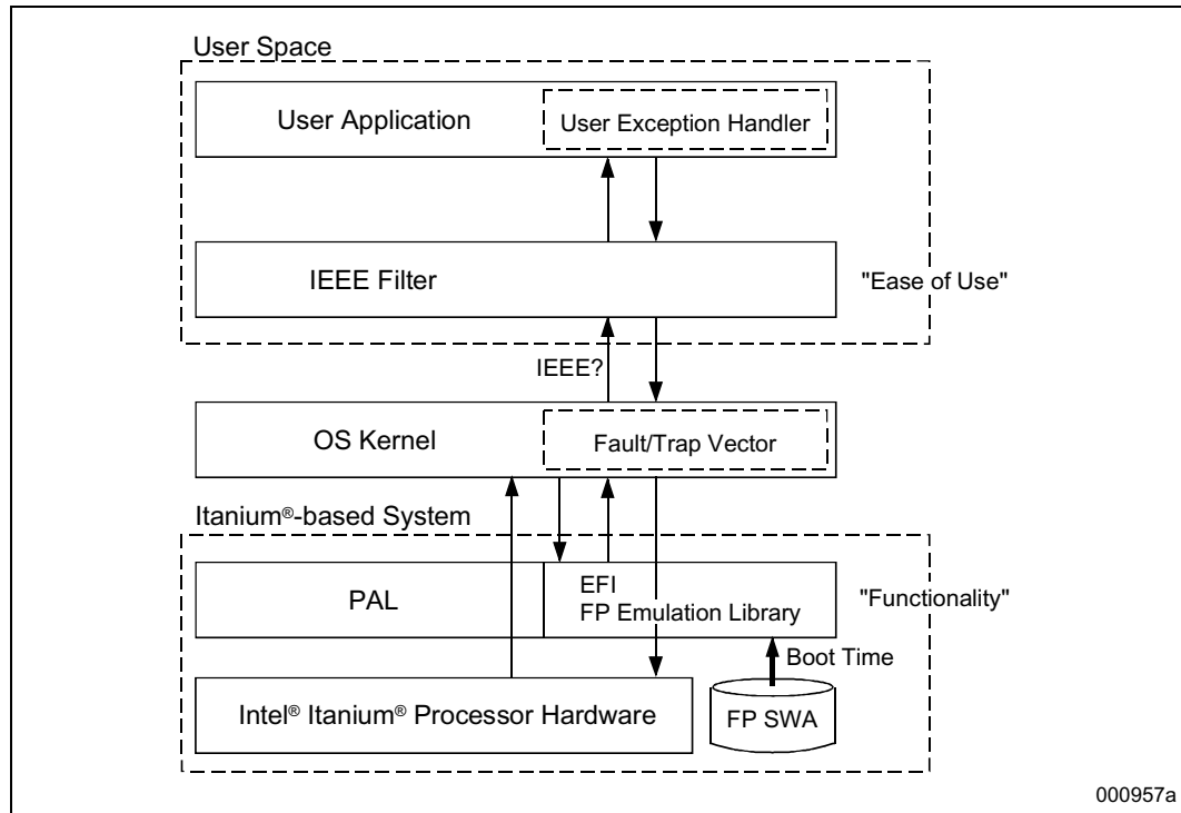
Figure 8-1. Overview of Floating-point Exception Handling in the Intel® Itanium® Architecture
