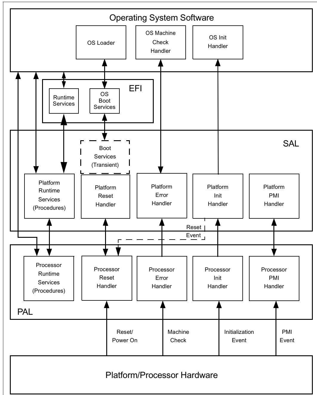
Figure 11-2. Firmware Services Model
