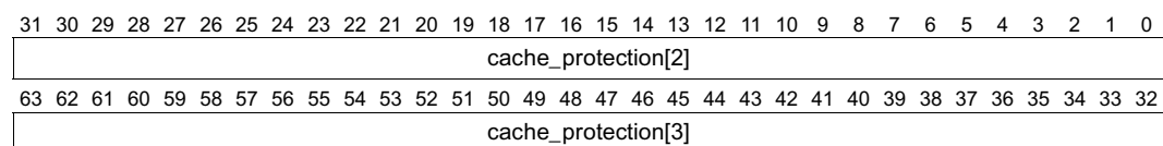
Figure 11-23. config_info_2 Return Value
