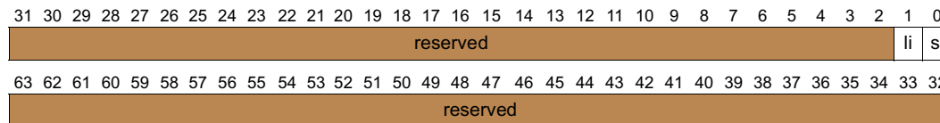
Figure 11-44. Layout of hints Return Value
