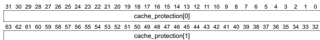
Figure 11-22. config_info_1 Return Value
