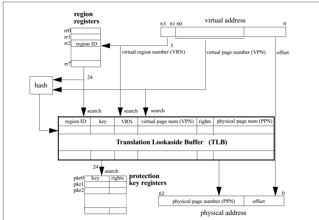
Figure 4-2. Conceptual Virtual Address Translation for References
