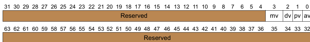
Figure 11-51. Layout of TR_valid Return Value
