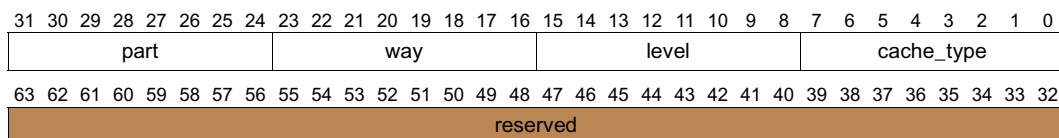
Figure 11-25. Layout of line_id Return Value
