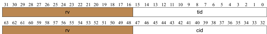
Figure 11-33. Layout of proc_n_log_info1 Return Value
