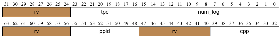
Figure 11-32. Layout of log_overview Return Value
