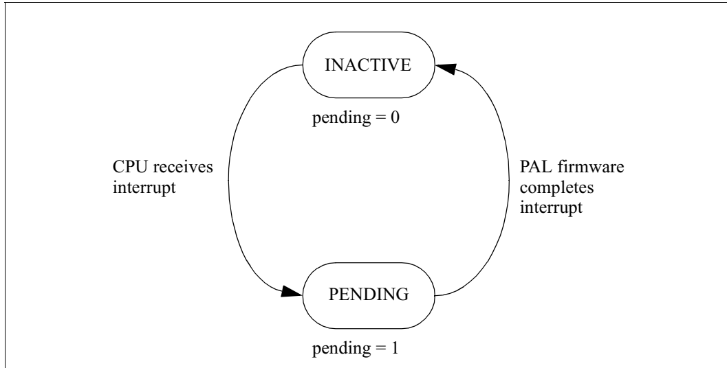
Figure 5-5. External Interrupt States
