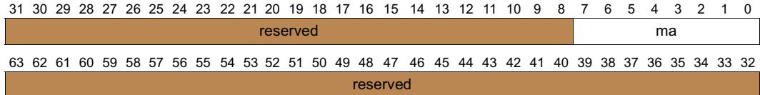
Figure 11-42. Layout of attrib Return Value
