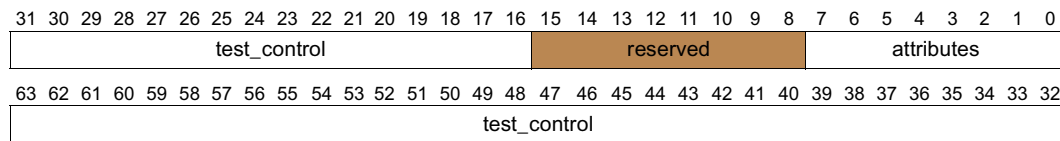
Figure 11-46. Layout of test_param Argument
