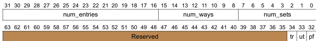
Figure 11-48. Layout of tc_info Return Value
