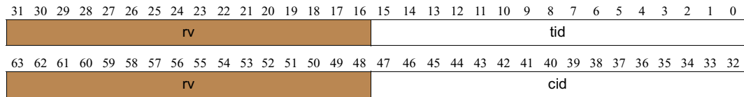
Figure 11-26. Layout of proc_n_log_info1 Return Value
