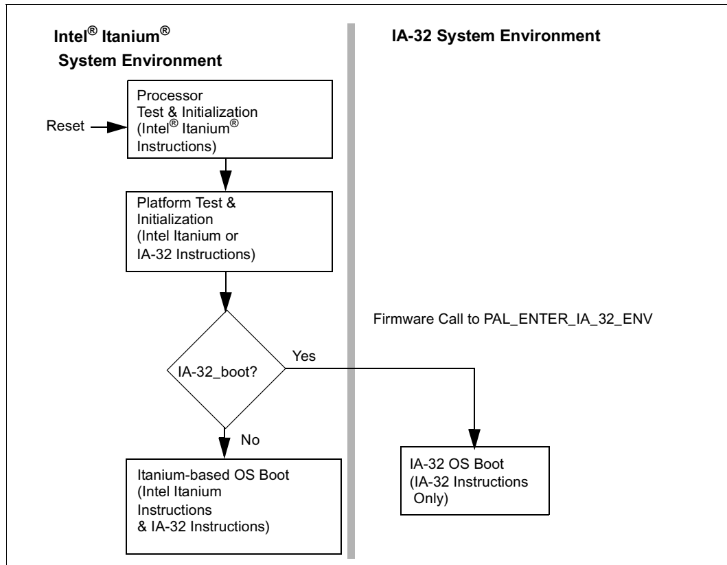
Figure 2-1. System Environment Boot Flow
