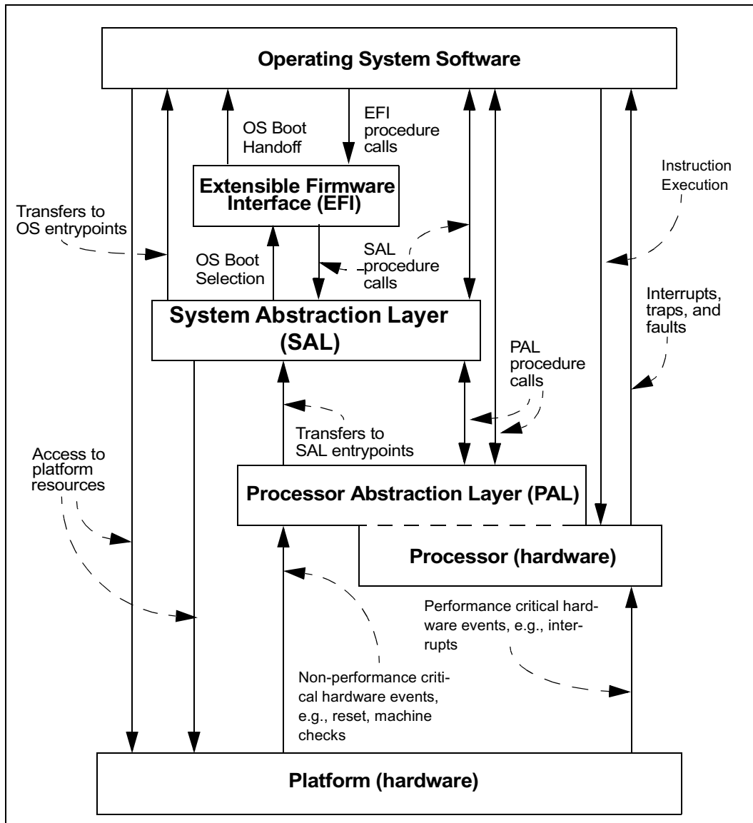
Figure 11-1. Firmware Model
