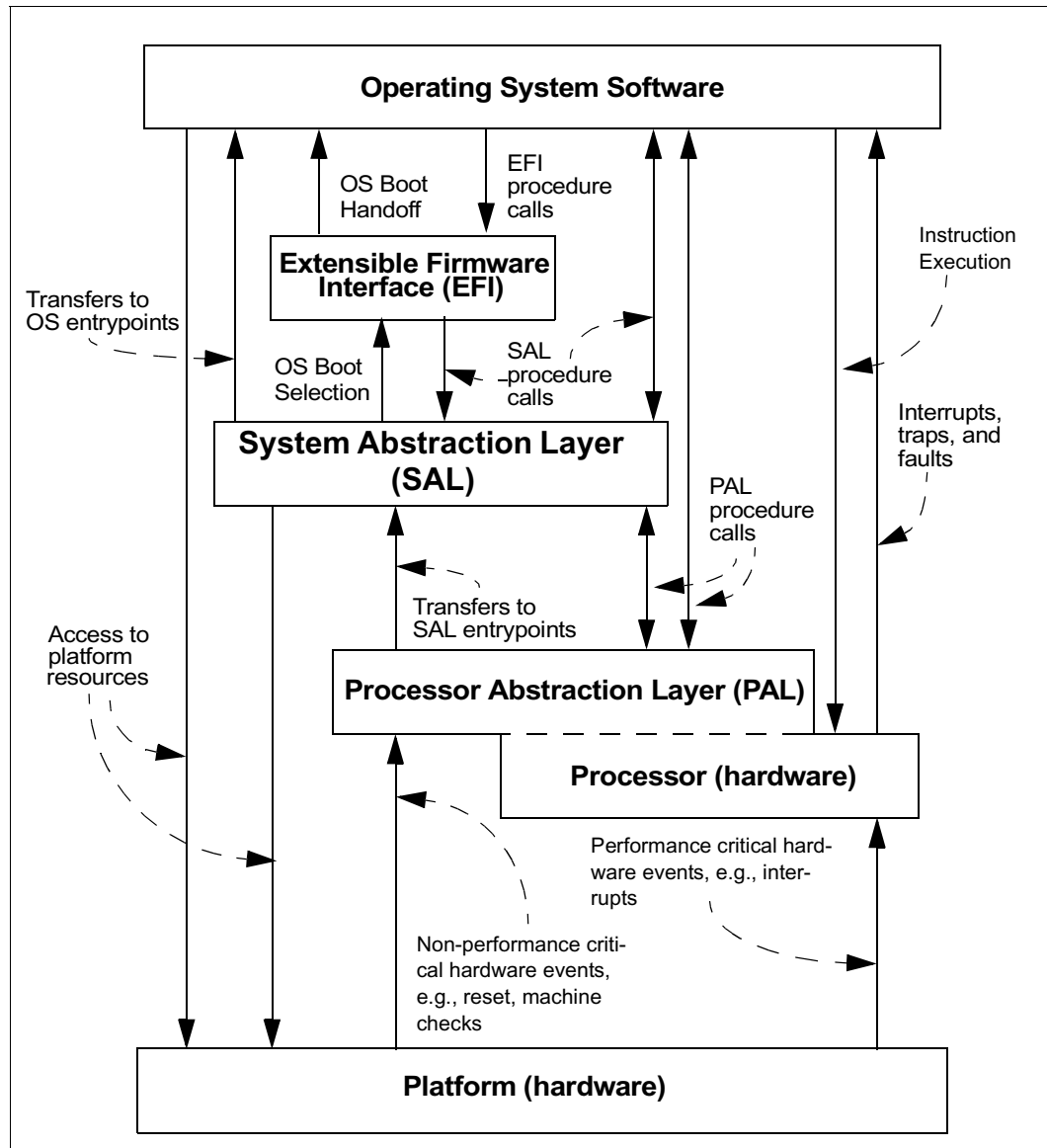
Figure 13-1. Firmware Model
