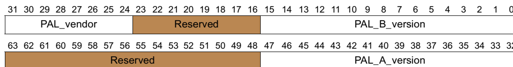
Figure 11-47. Layout of min_pal_ver and current_pal_ver Return Values
