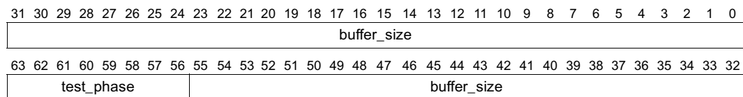
Figure 11-45. Layout of test_info Argument
