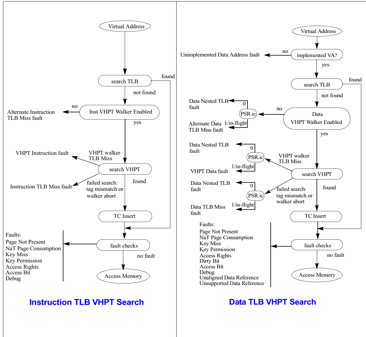
Figure 4-16. TLB/VHPT Search
