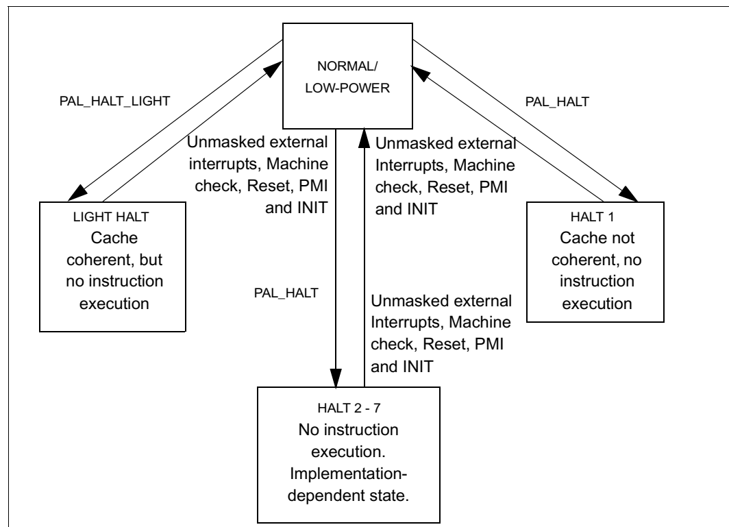
Figure 11-18. Power States
