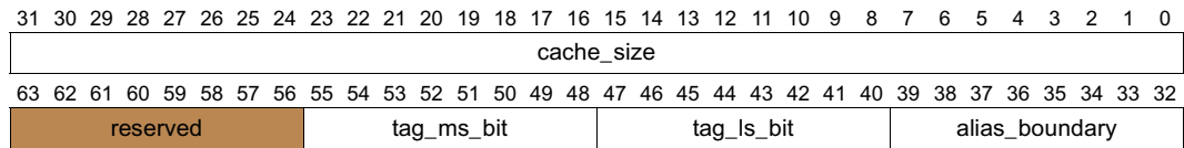
Figure 11-21. config_info_2 Return Value
