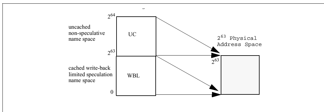
Figure 4-21. Addressing Memory Attributes
