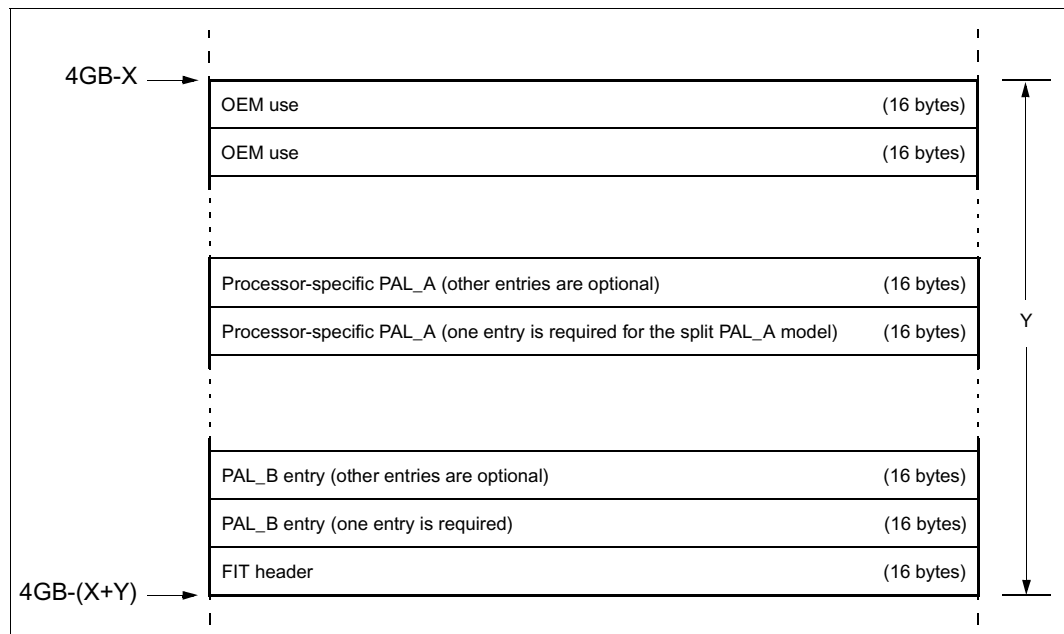
Figure 11-6. Firmware Interface Table
