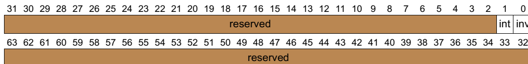
Figure 11-19. operation Parameter Layout
