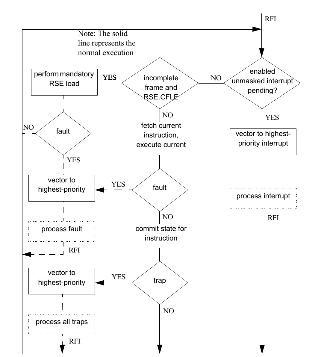
Figure 5-2. Interruption Processing
