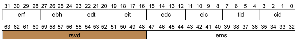
Figure 11-36. level_index Layout
