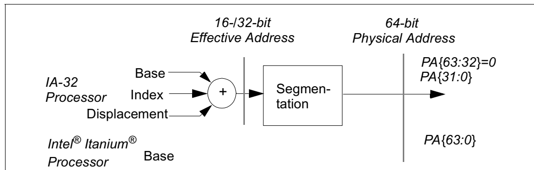
Figure 10-5. Physical Memory Addressing
