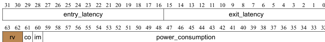
Figure 11-31. Layout of power_buffer Return Value
