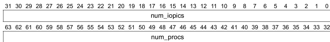
Figure 11-29. Layout of platform_info Input Parameter
