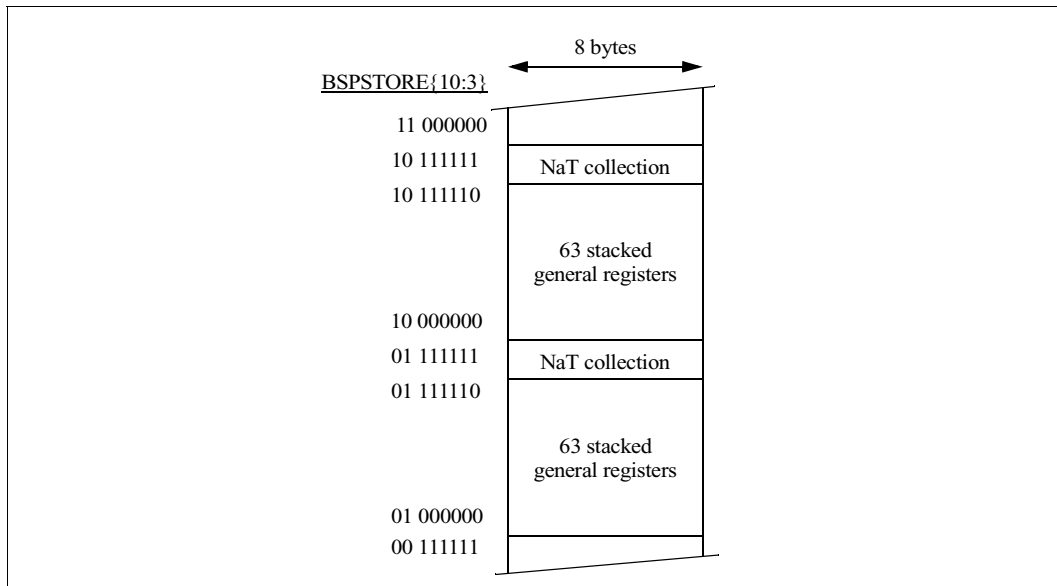
Figure 6-2. Backing Store Memory Format
