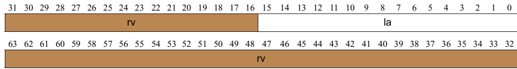
Figure 11-34. Layout of proc_n_log_info2 Return Value
