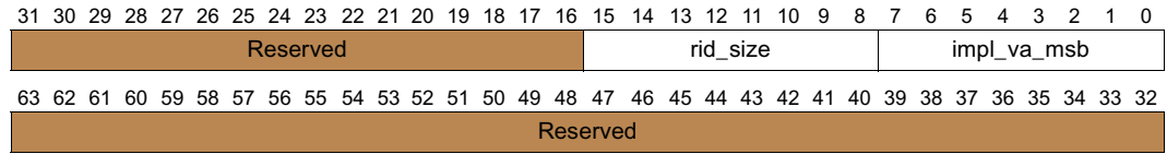
Figure 11-50. Layout of vm_info_2 Return Value
