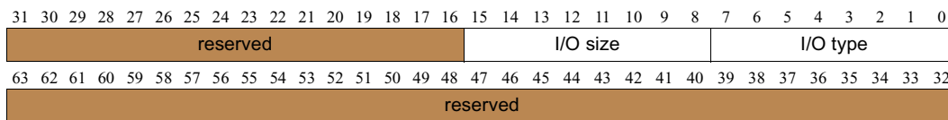
Figure 11-30. I/O Size and Type Information Layout
