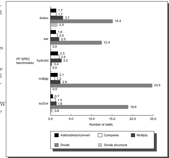
EE 4720 FIGURE 3.48 Stalls per FP operation for each major type of FP operation.
