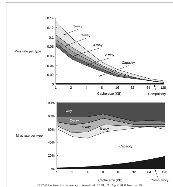
FIGURE 5.10 Total miss rate (top) and distribution of miss rate (bottom) for each size cache according to three C's for the data in Figure 5.9.
