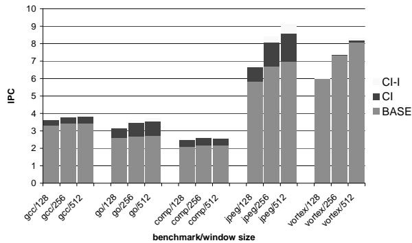
FIGURE 5. Performance of the three models.
