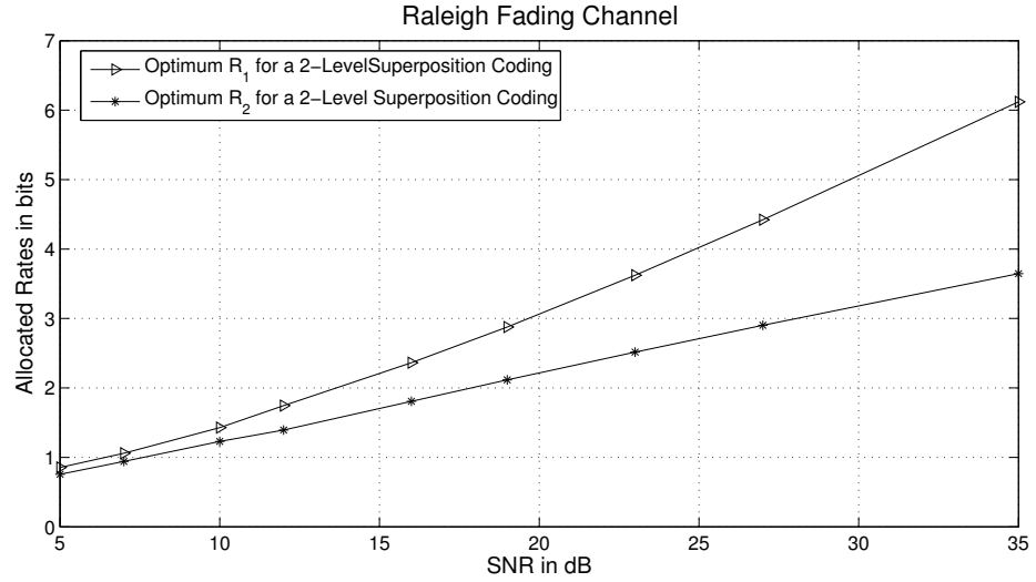
FIGURE 5.2. The value of rates R_1 and R_2 with SNR in a Direct Transmission
