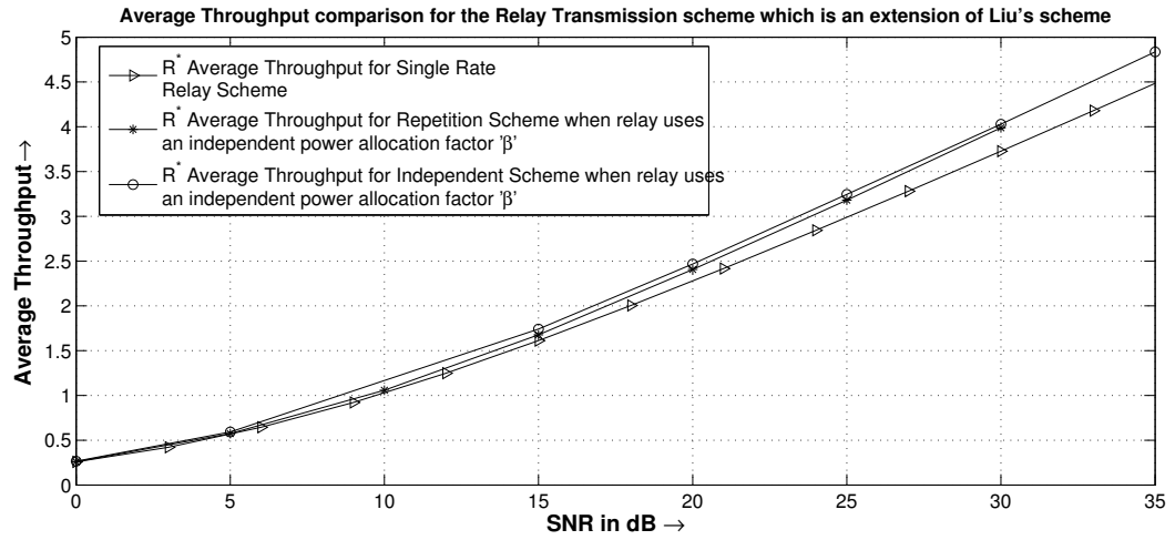
FIGURE 5.8. Comparison of Average throughput when relay uses Successive Interference cancellation method
