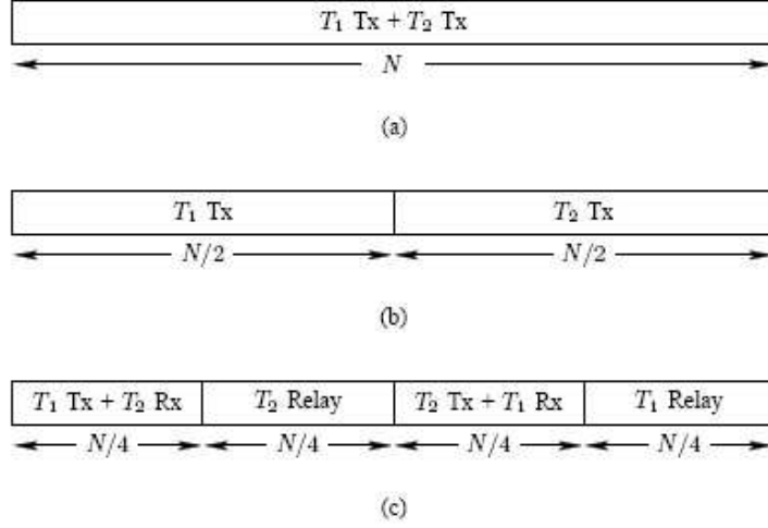
FIGURE 1.3. Time-division channel allocation for (a) direct transmission with interference, (b) orthogonal direct transmission, and (c) orthogonal cooperative diversity. This figure was adapted from [3]
