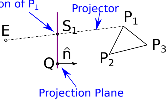
P_1, P_2, P_3 in 3D Coordinates
