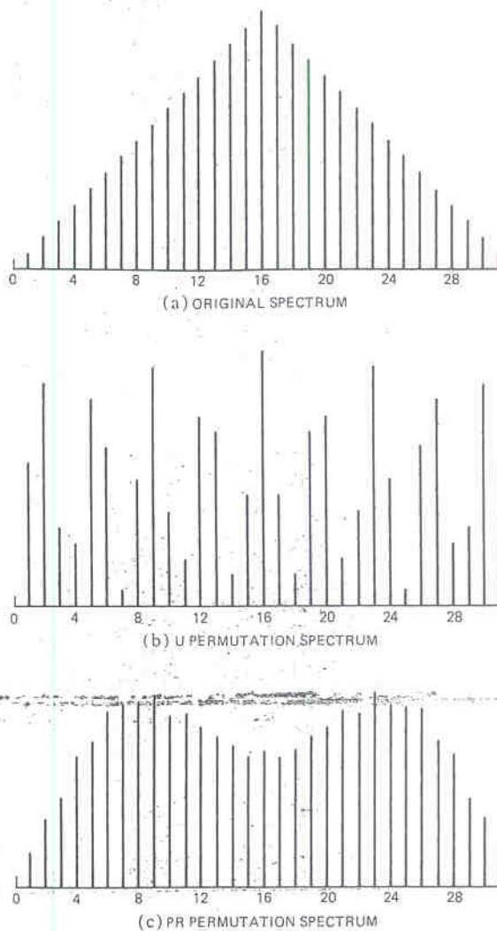
Fig. 5—Effects of PR and U permutation on high-pass spectrum.
