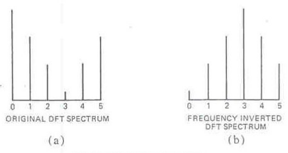
Fig. 8—Frequency inversion.
