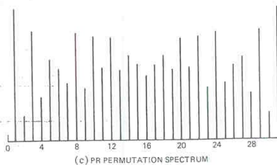
Fig. 6—Effects of PR and U permutations on mid-pass spectrum.
