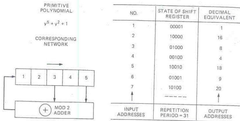
Fig. 1—Pseudorandom scrambler with a five-stage shift register.
