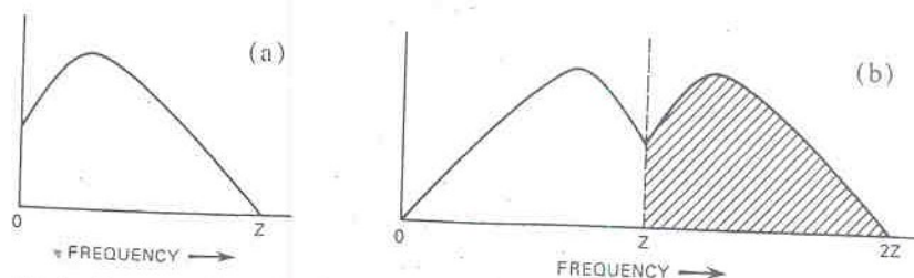
Fig. 9—Frequency inversion by modulation and low-pass filtering. (a) Original band-limited spectrum. (b) Result of modulating spectrum with carrier at Z . The left half of (b) is the inverse of (a).
