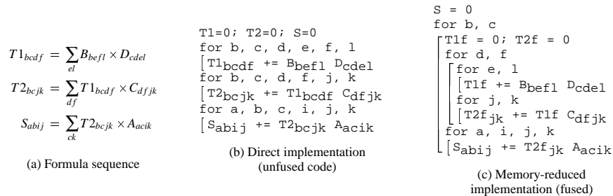
Fig. 2. Example illustrating use of loop fusion for memory reduction.
