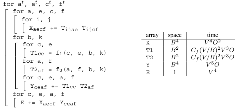
Figure 4. Use of tiling and partial fusion to reduce recomputation cost.
