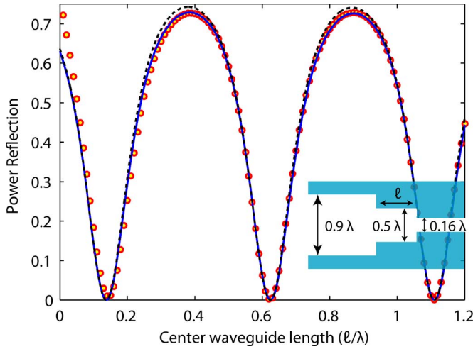
Fig. 5. Test of the scattering matrix description. Horizontal axis is the length of the center waveguide normalized to \lambda . Vertical axis is the power reflection coefficient. FDTD simulation results ( \bullet ), transfer matrix calculations using lossy junctions (solid line) and lossless junctions (dashed line) are also plotted. Transfer matrix calculations do take into account the loss in the center waveguide for both cases. As the junctions get very close to each other ( < 0.1\lambda ), transfer matrix model begins to break down due to higher order modal interactions.
