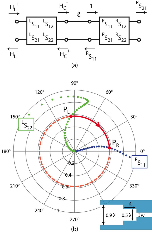
Fig. 4. (a) Schematic diagram of modal propagation. The left and right junctions are shown as boxes with an S matrix description. The center waveguide is shown as a transmission line of length \ell . The source that creates the fields is normalized such that the mode that propagates to the right has a unit magnitude at the input of the right junction. (b) Graphical solution of (11) and (12) on the complex plane. Point P_L is the location of the left junction on the L_{S_{22}} curve where b = 0.9\lambda and b' = 0.5\lambda . Point P_R is the location of the right junction on the R_{S_{11}} curve where b = 0.5\lambda and b' = 0.16\lambda .
